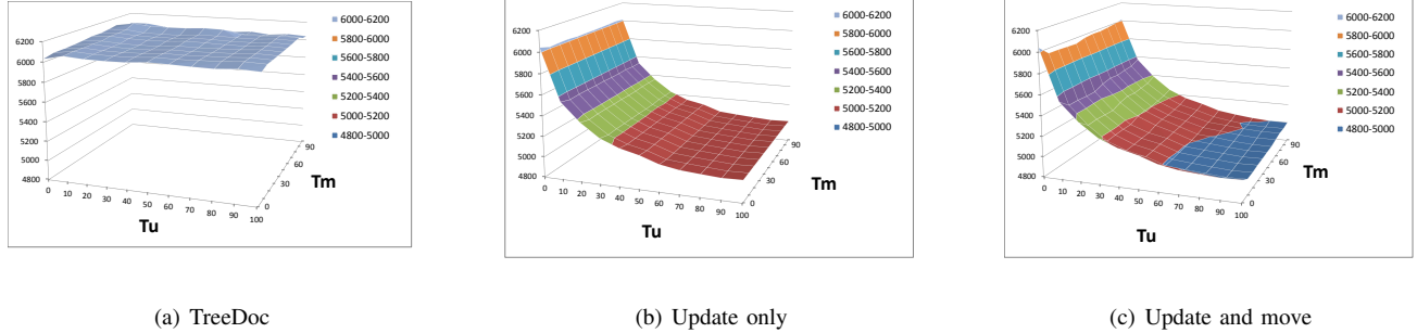
Fig. 3. Threshold effect
