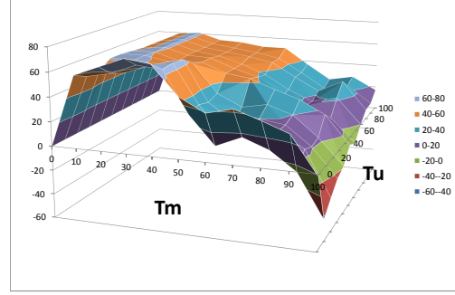
Fig. 4. Move effect
