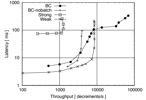
Fig. 7: Throughput vs. latency with multiple counters.
