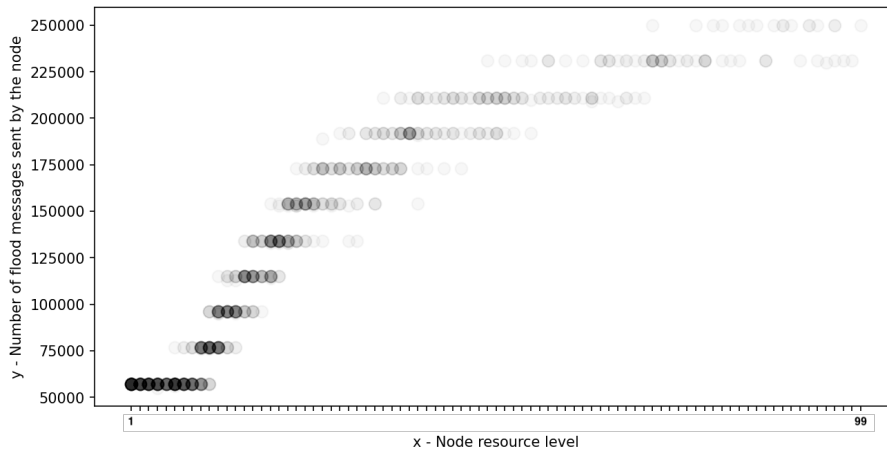
Figure 5.8: Load per node capacity of our solution prototype using Proteus average mode, with the lognormal distribution.
