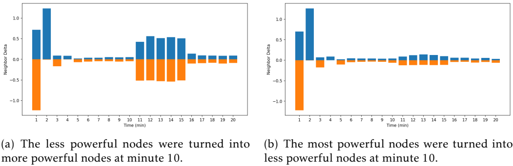
Figure 5.10: Average number of neighbors variability over time while modifying node resources mid-execution, while using Proteus average mode.
